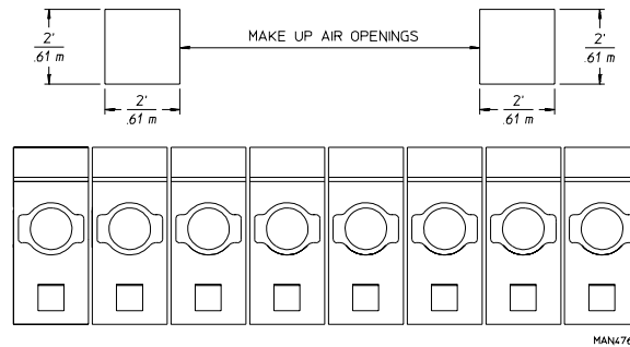
TYPICAL INSTALLATION SHOWING MAKE - UP AIR OPENINGS
